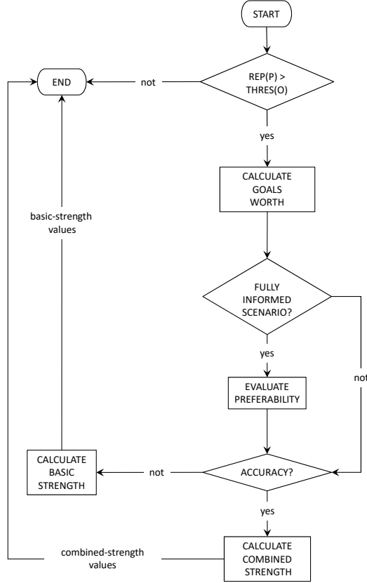
Figure 1: Work-flow of the proposed strength calculation model.
