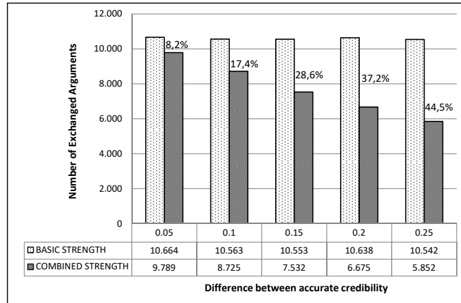
Figure 8: Experiment 4: comparison of the variable number of exchanged arguments .
