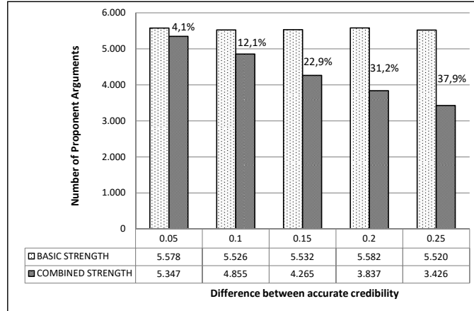
Figure 7: Experiment 4: comparison of the variable number of arguments sent by the proponent .
