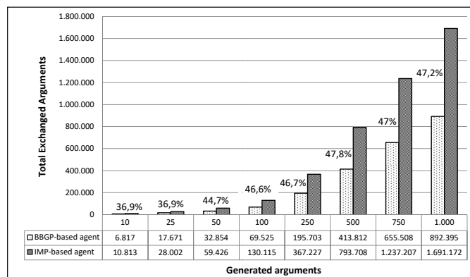
Figure 3: Experiment 1: Comparison of the variable number of exchanged arguments .
