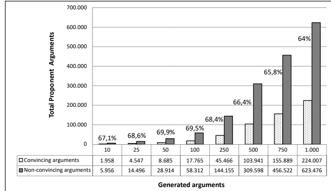
Figure 5: Experiment 2: Comparison of the variable number of arguments sent by the proponent .
