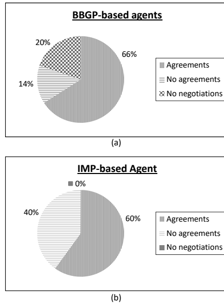
Figure 4: Percentage of negotiations that end in an agreement vs. percentage of negotiations that do not end in an agreement. (a) For BBGP-based agents. (b) For IMP-based agents.
