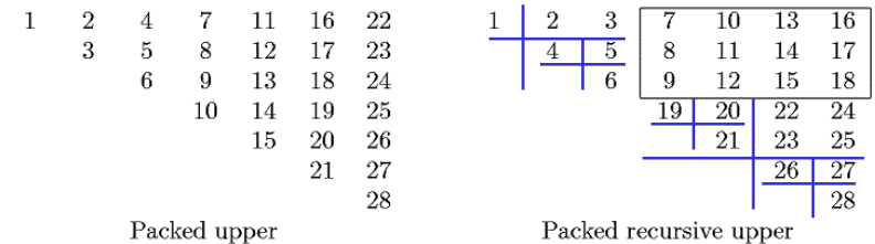
FIG. 3.1. Memory indices for 7 \times 7 upper triangular matrix stored in traditional packed format and recursive packed format.
