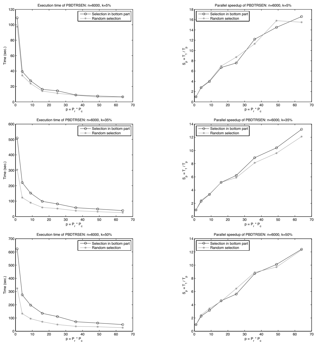
Figure 10. Experimental results for n = 6000 from Table II on seth . Displayed representative performance results are for different variations of the number of selected eigenvalues, their distribution over the diagonal of the Schur form and the number of utilized processors.
