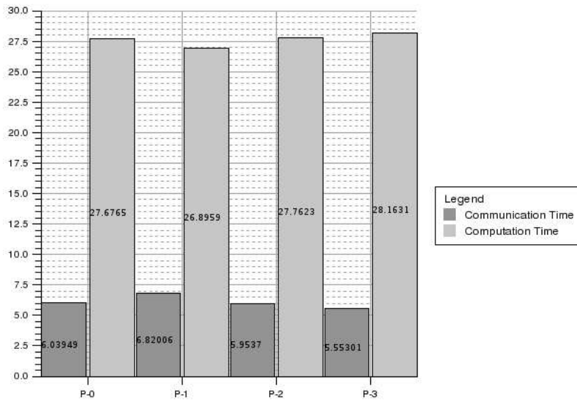
Figure 12. Execution time profile for four processors reordering 5% of the eigenvalues of a 6000 x 6000 matrix: total cost of computations vs communications.
